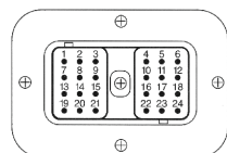
Flange Mount Receptacle
