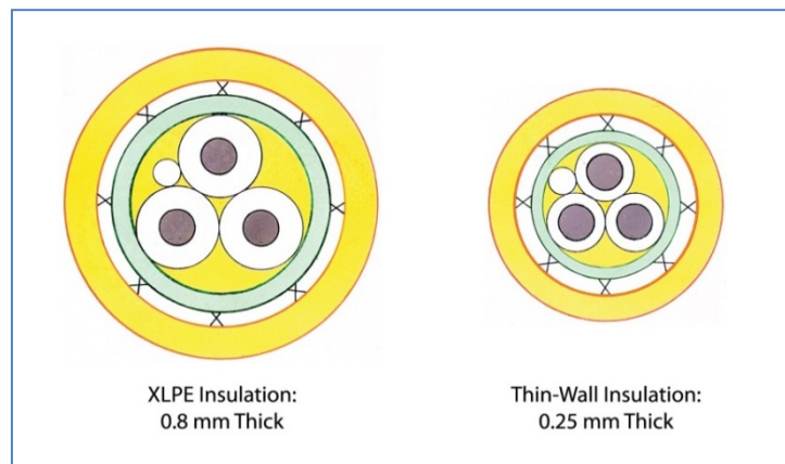
Fig. 2. TE Connectivity’s Raychem Thin-Wall Insulations Can Significantly Reduce Cable Size and Weight (Source: TE Connectivity)
