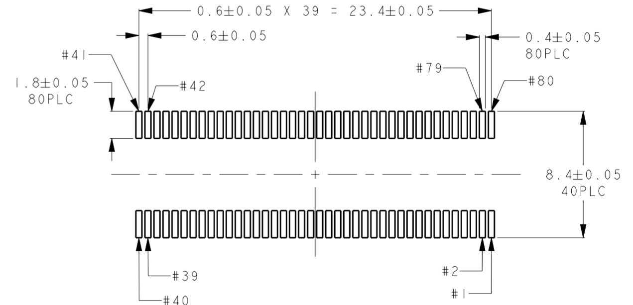
推奨基板取付寸法 RECOMMENDED PCB LAYOUT
