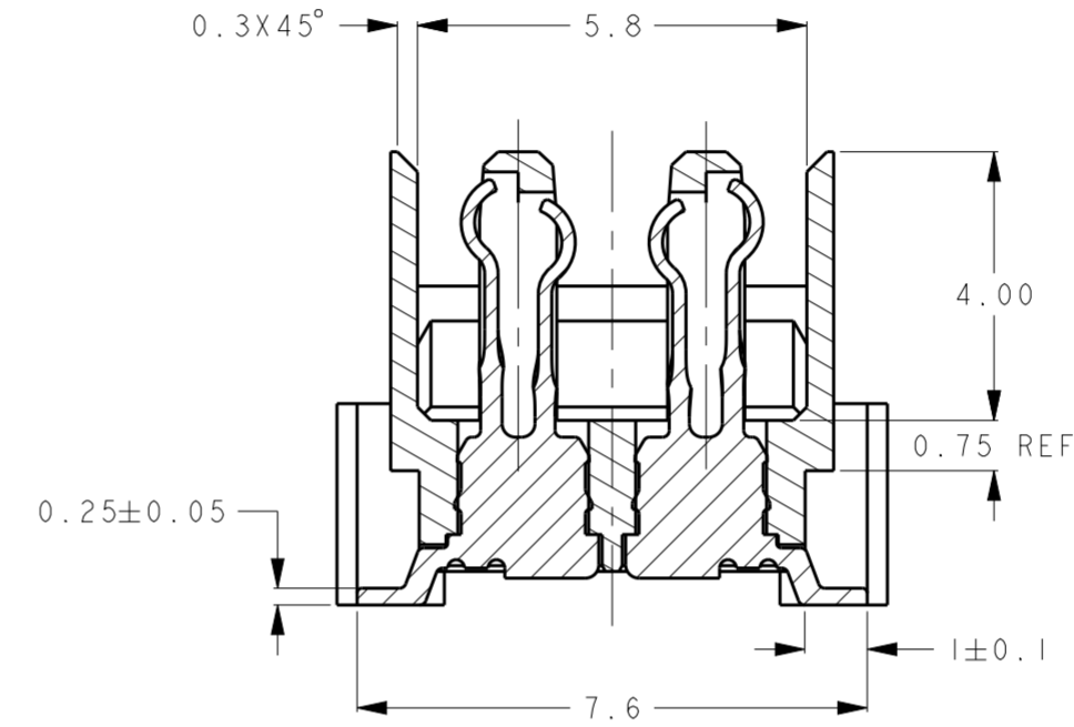
A - A SCALE 8:1
