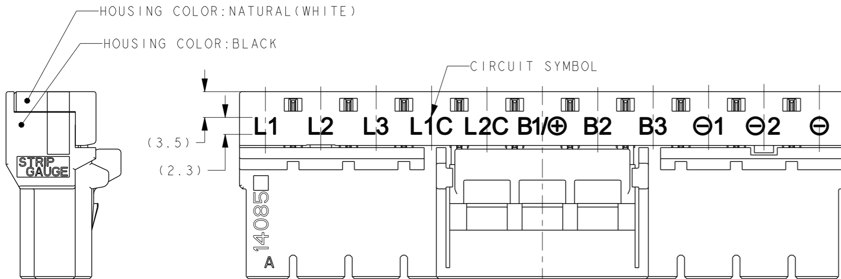
I-2289080-2 (11 POSITION KEYING: X)
