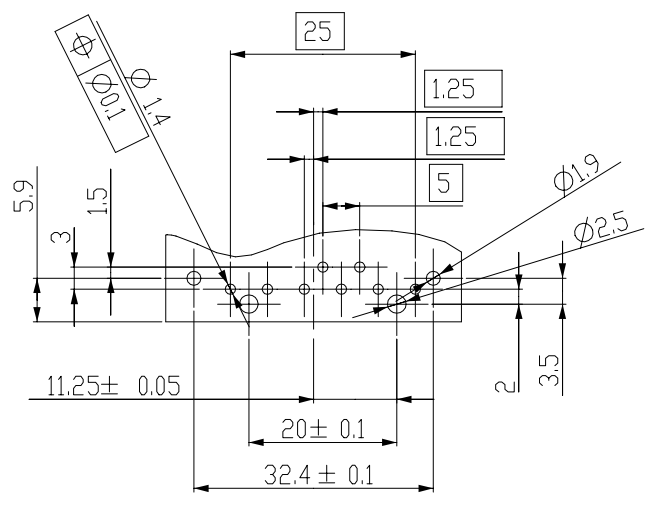
MOUNTING DIMENSION FOR P.C.B.
