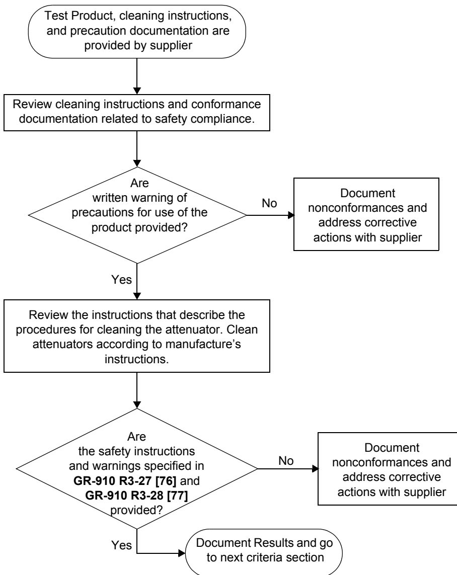
TP-910 Figure 3-8 Test Flowchart - Safety (not from GR-910)
