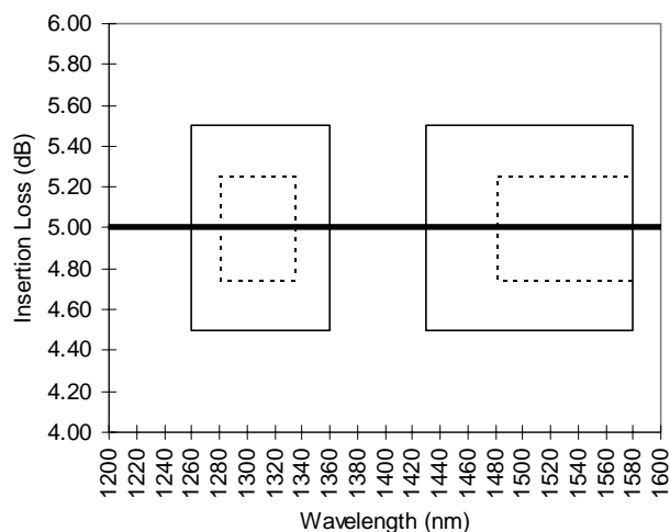
TP-910 Figure 4-102 5 dB Attenuator Optical Bandpass Spectra
