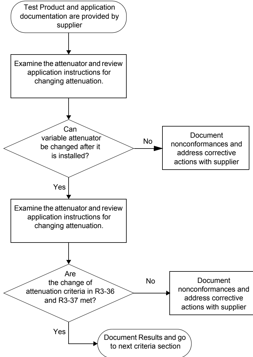
TP-910 Figure 3-11 Test Flowchart - Change of Attenuation (not from GR-910)
