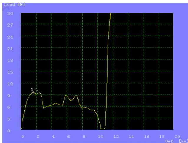
Figure 1- typical contact insertion force profile plot
