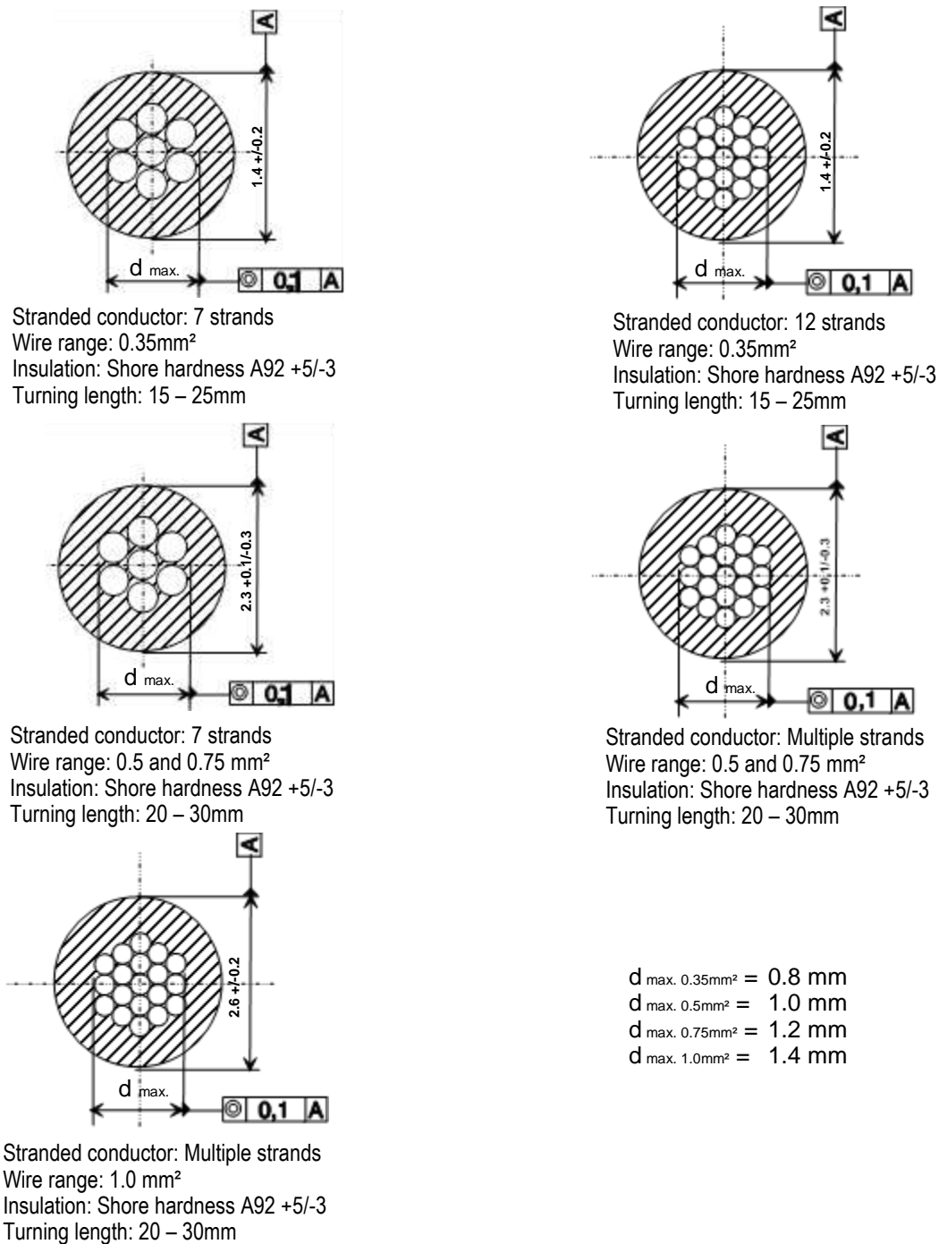
Figure 23: Typical Conductor Cross Sections
