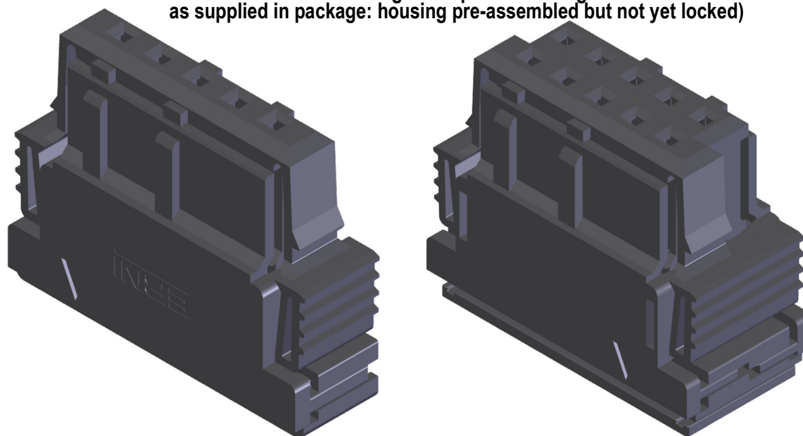
Figure 1 364226-E (single-row 5p) 474034-E (dual-row 10p)
