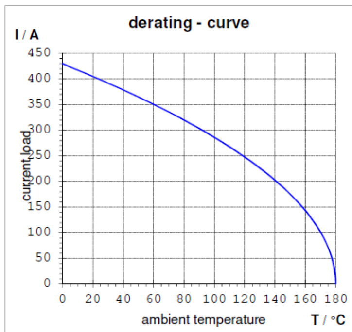
Figure 6: Derating curve 70mm 2 applied with 20%-Safety factor.
