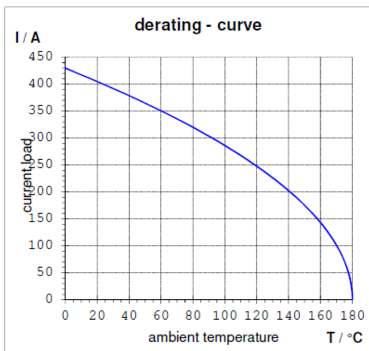
Figure 7: Derating curve 95mm 2 applied with 20%-Safety factor.
