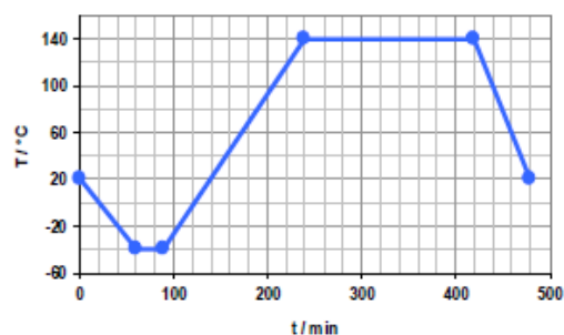
Figure 3 Temperature profile
