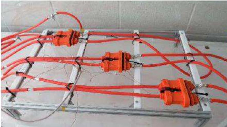
Figure 2: test setup housing influence on the derating
