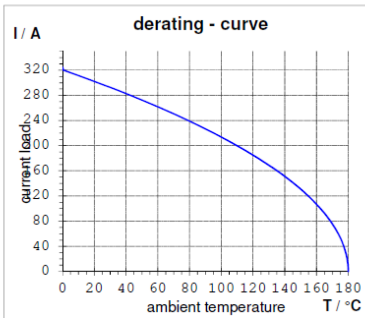
Figure 5: Derating curve 50mm 2 applied with 20%-Safety factor.
