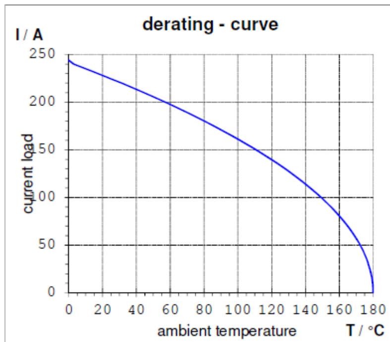
Figure 3: Derating curve 25mm 2 applied with 20%-Safety factor.
