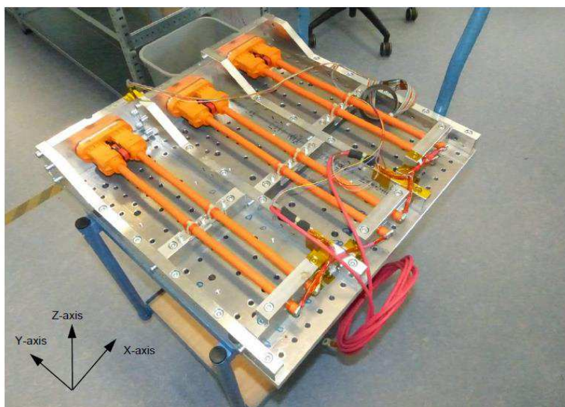
Figure 1 Test setup / overview of vibration directions.
