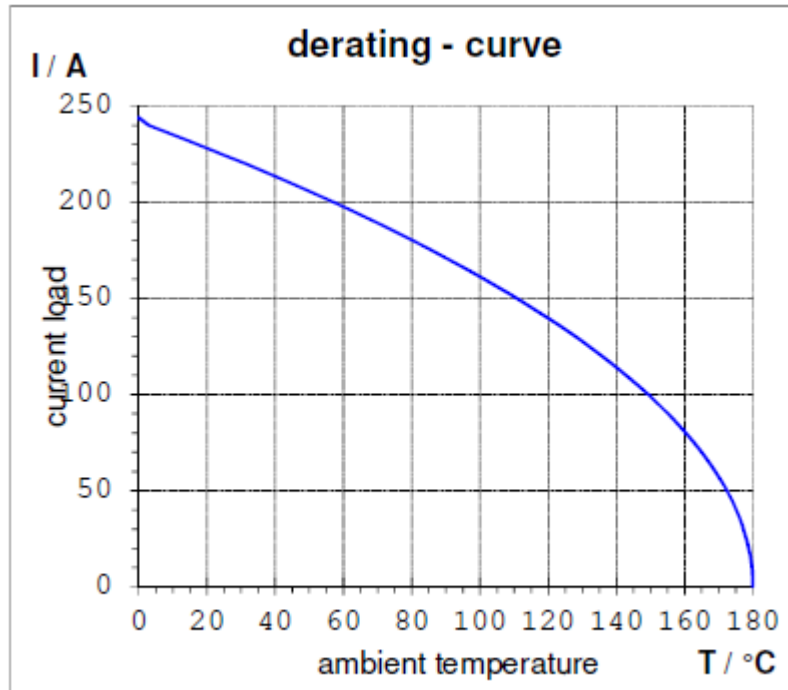
Figure 4: Derating curve 35mm 2 applied with 20%-Safety factor.
