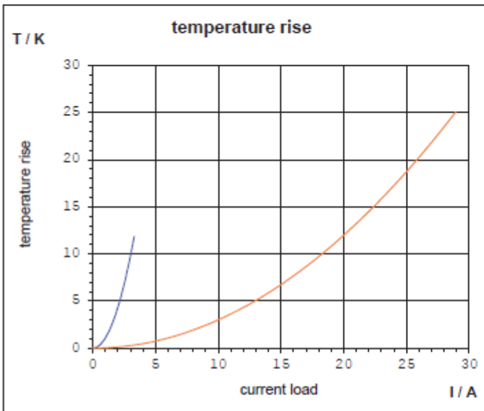
Figure 21 Temperature rise curve
