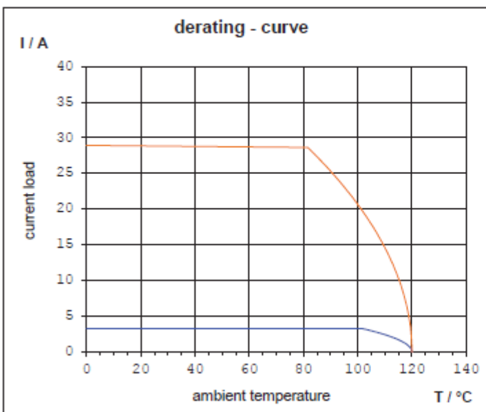
Figure 22 Derating curve
