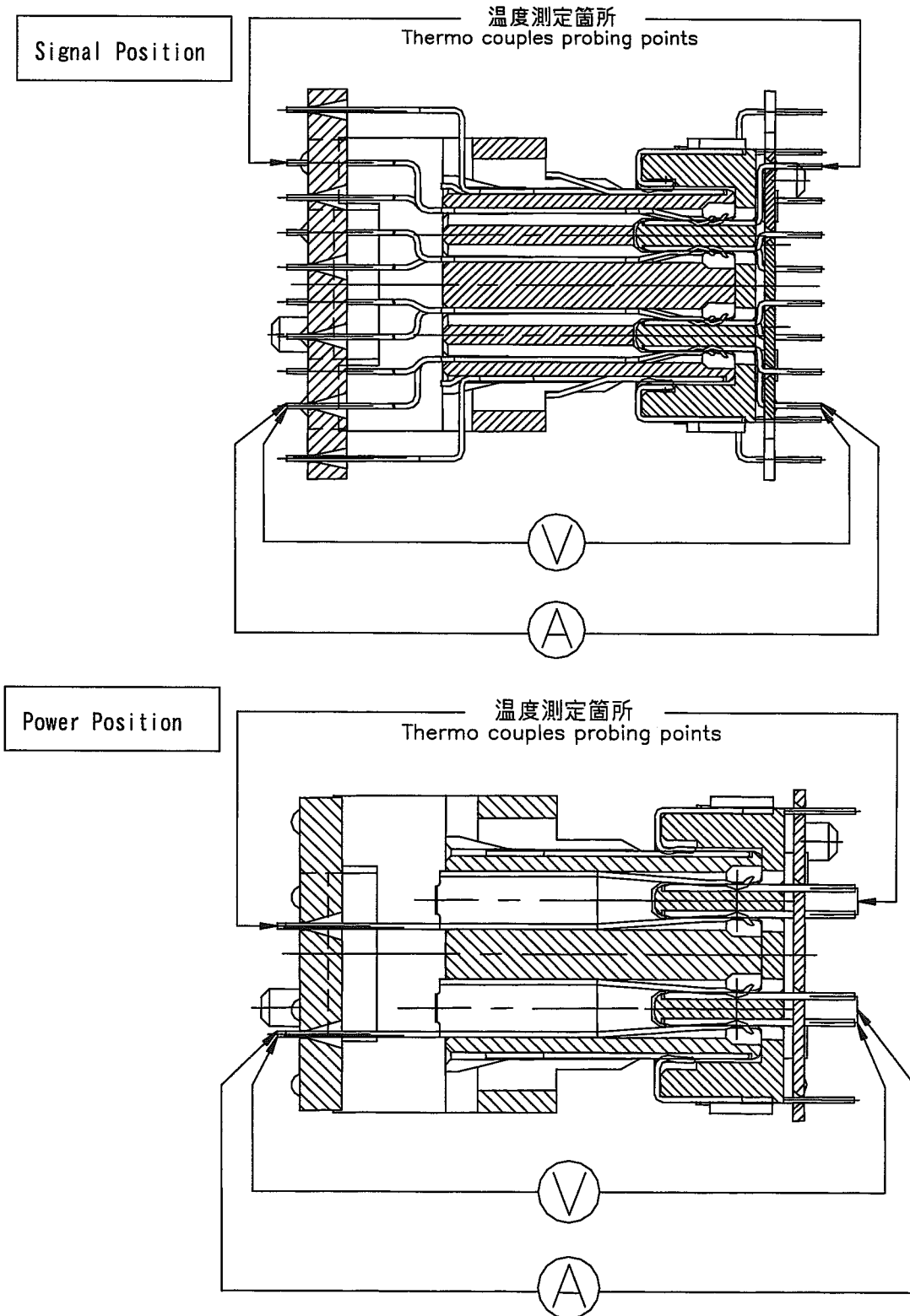
Fig. 3 0-VA 総合抵抗測定点 Fig3 Termination Resistance Measuring points
