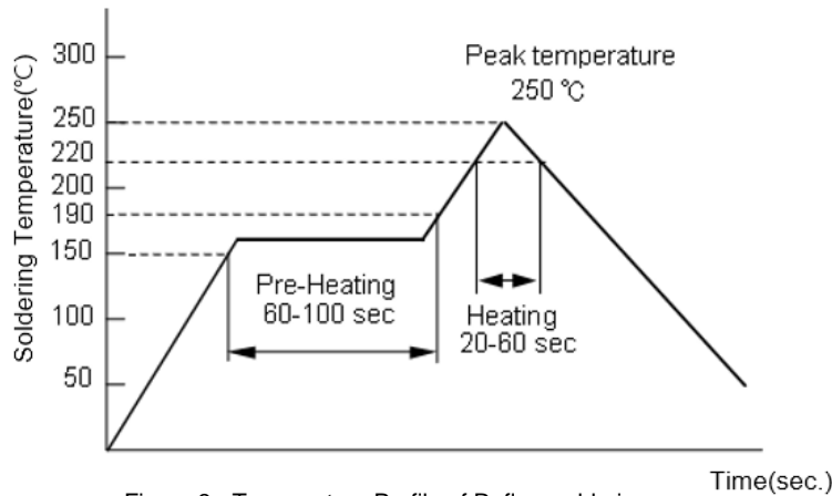
Figure 3 - Temperature Profile of Reflow soldering
