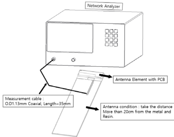
Figure 1 - VSWR Test
