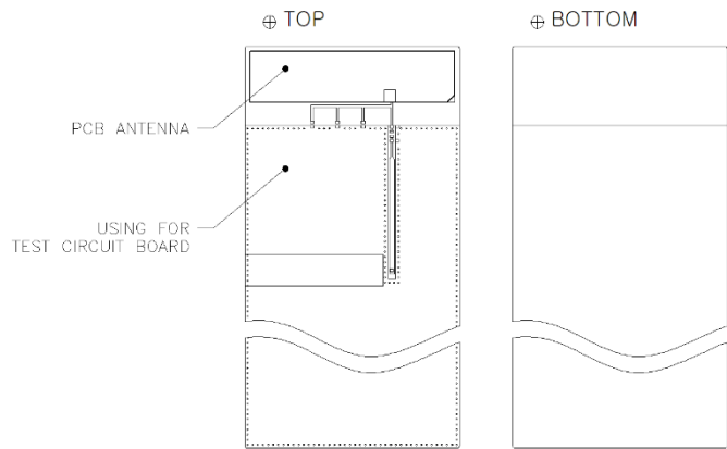
Figure 2 - Mounted PCB for V.S.W.R test
