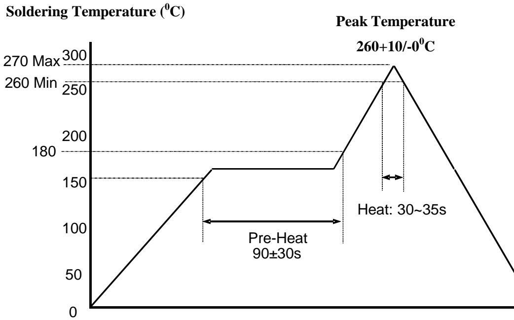
Figure 3 Temperature Profile for Reflow-Soldering
