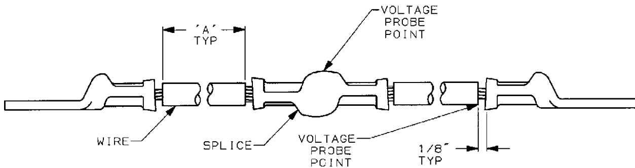
Voltage Probe Points For Splices
