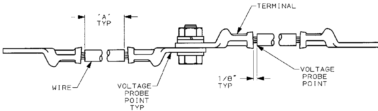
Voltage Probe Points For Terminals
