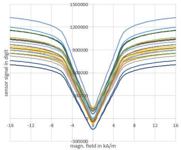
MD47 - sensor signals - offset calibrated
