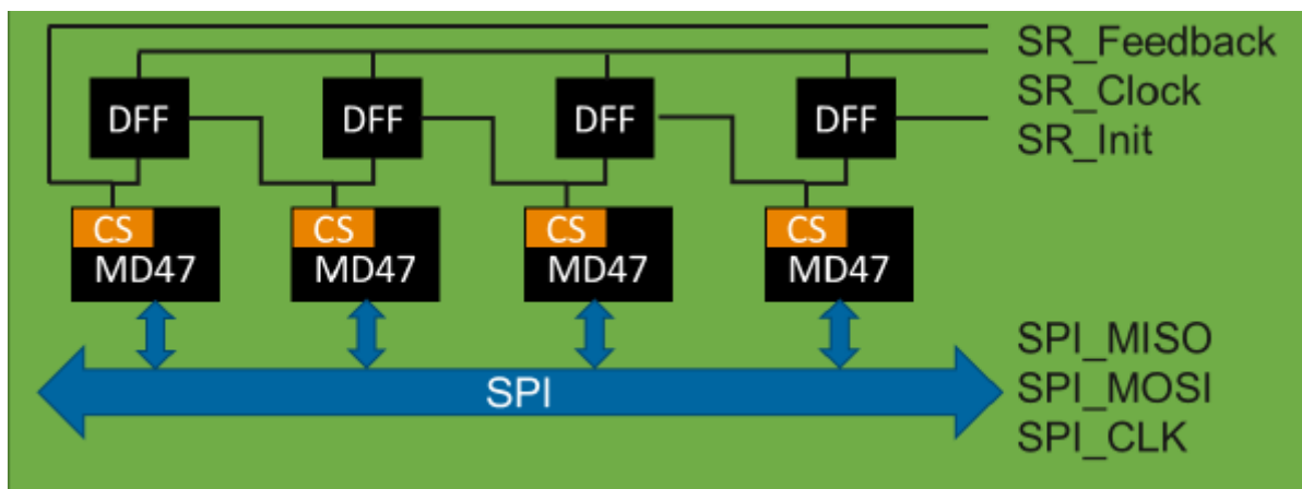
Figure 6: Block diagram of SPI Communication example
