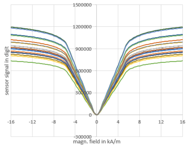
MD47 - sensor signals - offset and offset-TC calibrated
