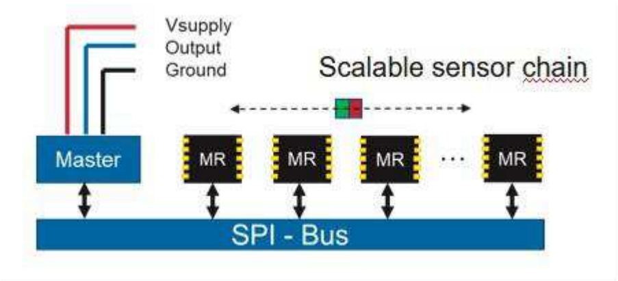
Figure 7: Scaleable Sensor Chain controlled by maste MCU
