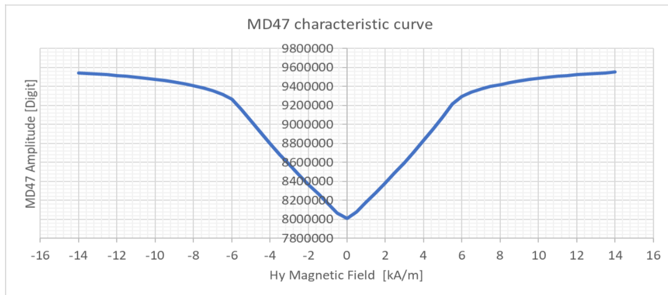
Figure 3: MD47 characteristic magnetic output curve
