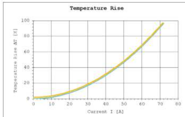
Curve 4: 2Pos connector with 6.0mm 2 wire
