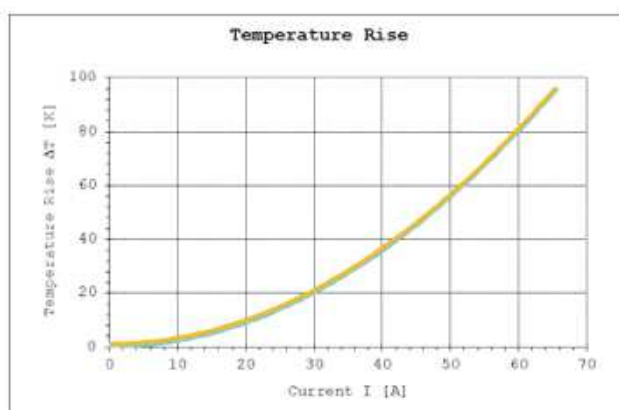
Curve 1: 3Pos connector with 6.0mm 2 wire
