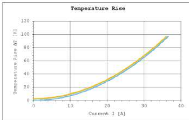
Curve 3: 3Pos connector with 2.5mm 2 wire
