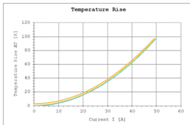
Curve 5: 2Pos connector with 4.0mm 2 wire
