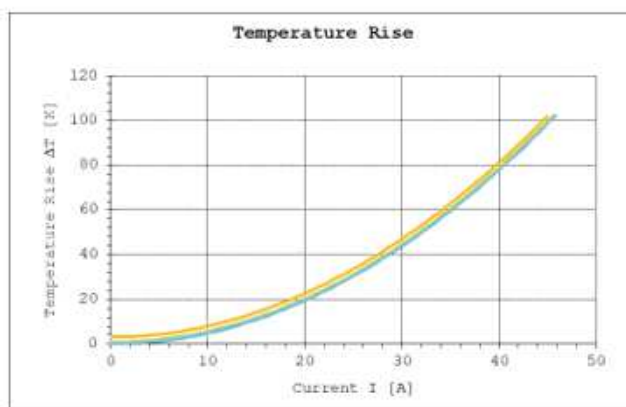
Curve 2: 3Pos connector with 4.0mm 2 wire
