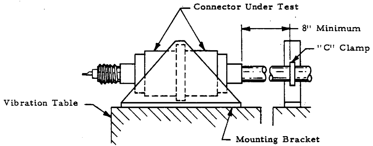
Figure 4 Vibration & Mechanical Shock Mounting Fixture
