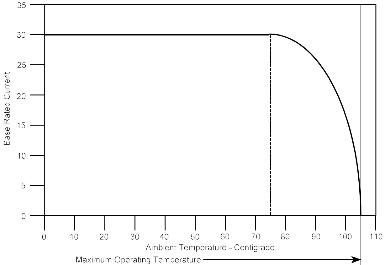
Rated Current vs Ambient Temperature Rating for Single Circuit I_{rms} or I_{dc} , Maximum Wire Gage, Continuous Operating
