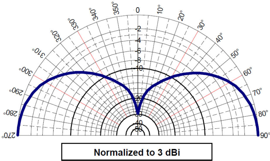
Elevation Pattern (Y, Z or H-plane)
