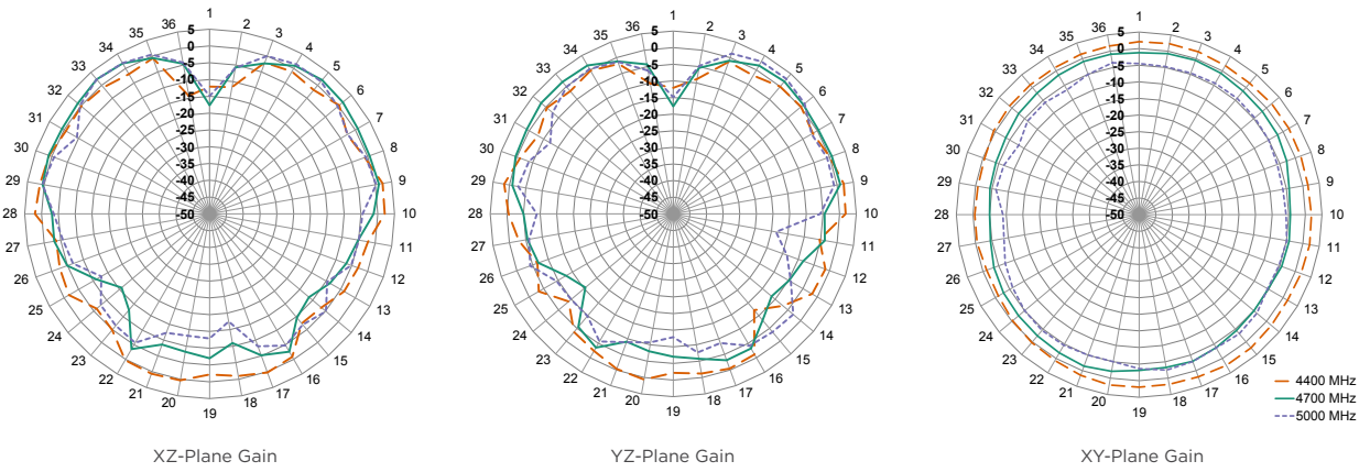
Figure 9. Radiation Patterns for ANT-5GWWS3-SMA, Straight
