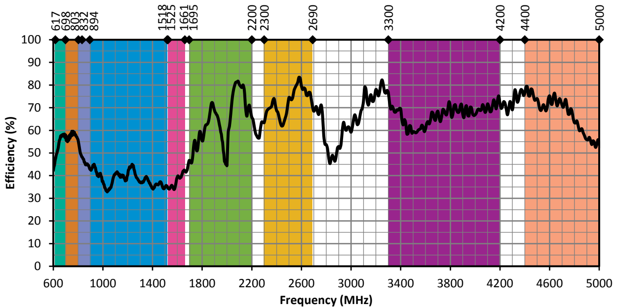
Figure 8. ANT-5GWWS3-SMA Antenna Efficiency, Straight
