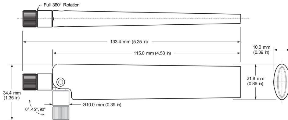
Figure 1. ANT-5GWWS3-SMA Antenna Dimensions
