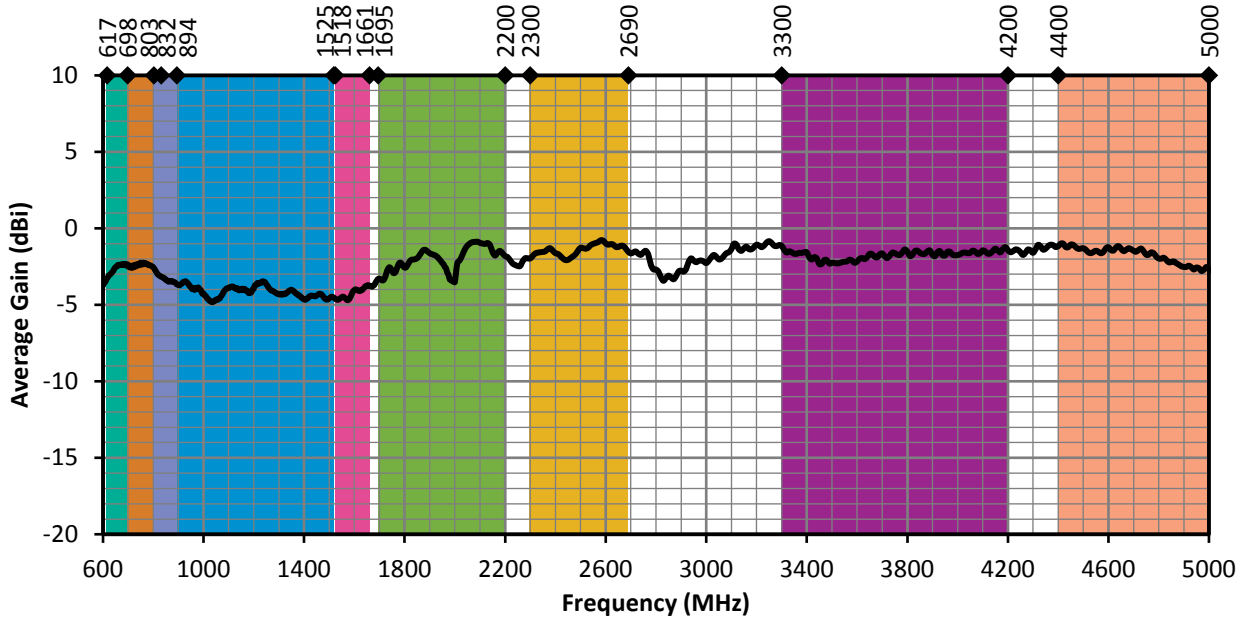
Figure 7. ANT-5GWWS3-SMA Antenna Average Gain, Straight
