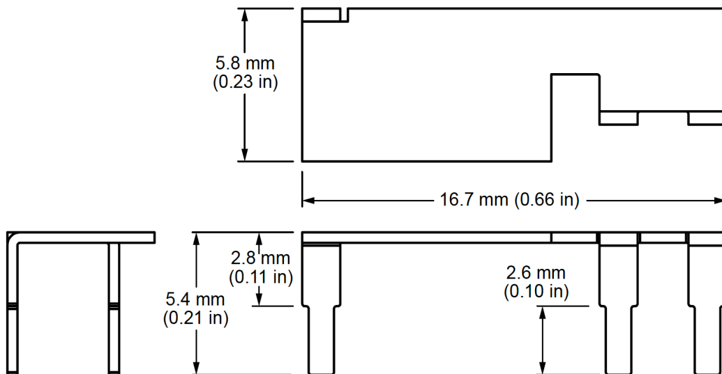
Figure 1. ANT-2.4-MSA-TH1 Antenna Dimensions
