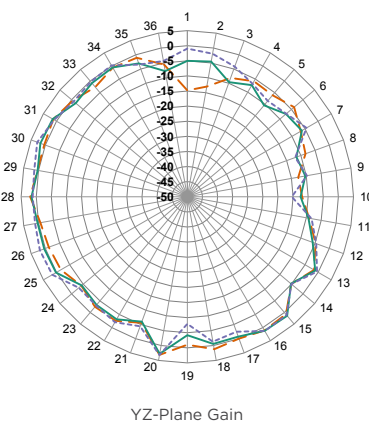
Figure 8. ANT-2.4-MSA-TH1 Antenna Radiation Patterns
