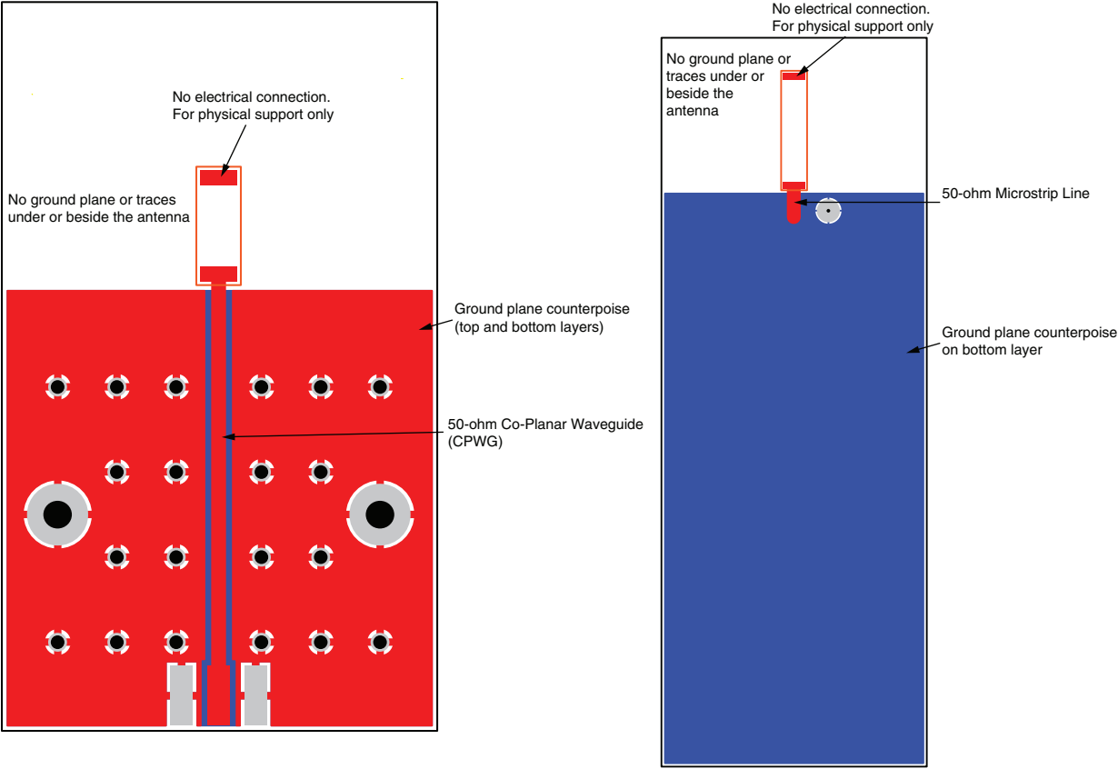
Figure 3: The CHP Series Test Fixtures
