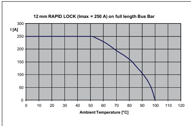
Figure 2a : RAPID LOCK Connector Derating Curve
