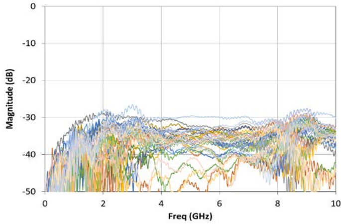
Return Loss (SDD11) of 1m 33AWG 100 Ohm 12G Sliver
