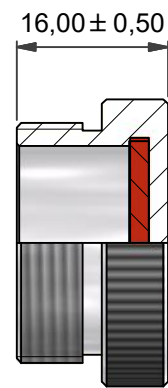
100P1167-16-1-C NO ATTACHMENT VERSION
