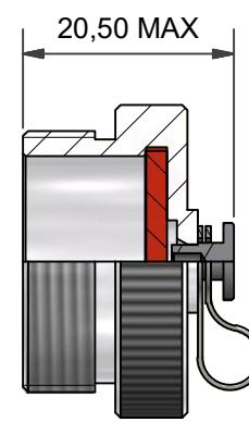
100P1167-16-1-C-EO EYELET ONLY VERSION (NO LANYARD)
