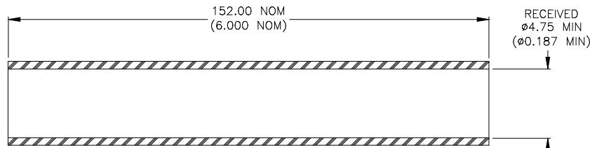
1) SLEEVE, OUTER COVER, Qty/kit: 1
