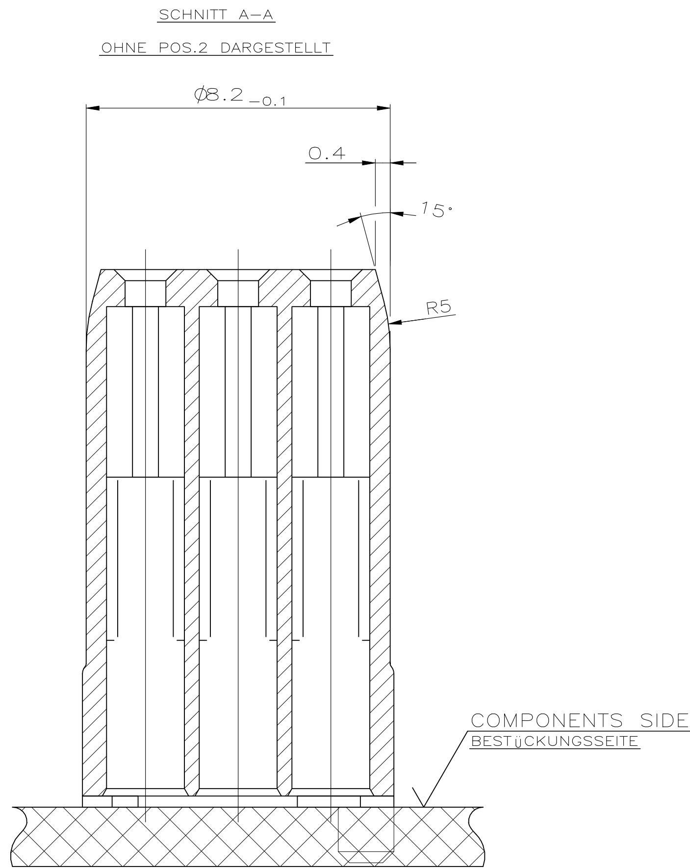
SECTION A-A SHOWN WITHOUT ITEM NO. 2
