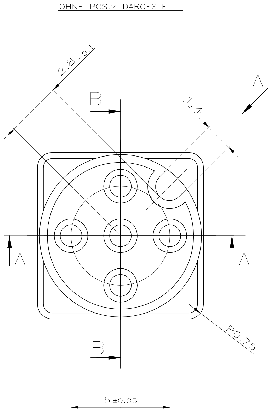
SHOWN WITHOUT ITEM NO. 2
