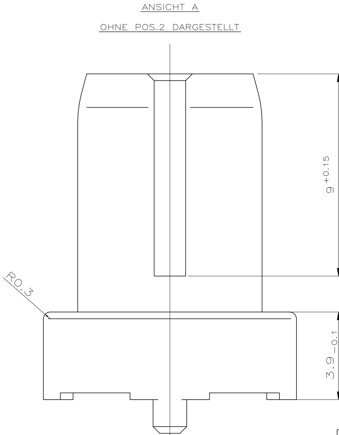
VIEW A SHOWN WITHOUT ITEM NO. 2
