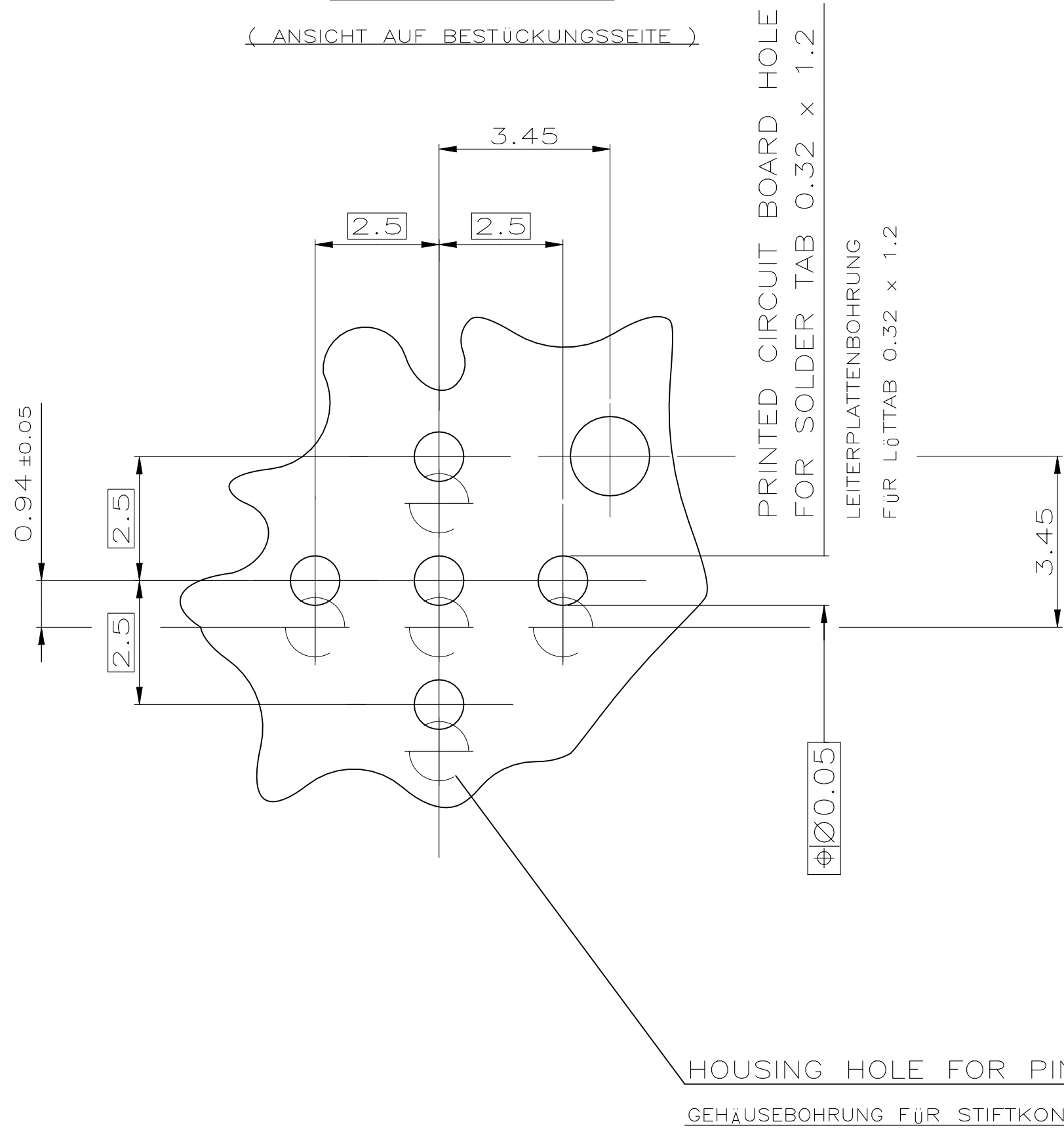
PRINTED CIRCUIT BOARD-LAYOUT ( VIEW ON COMPONENTS SIDE )
