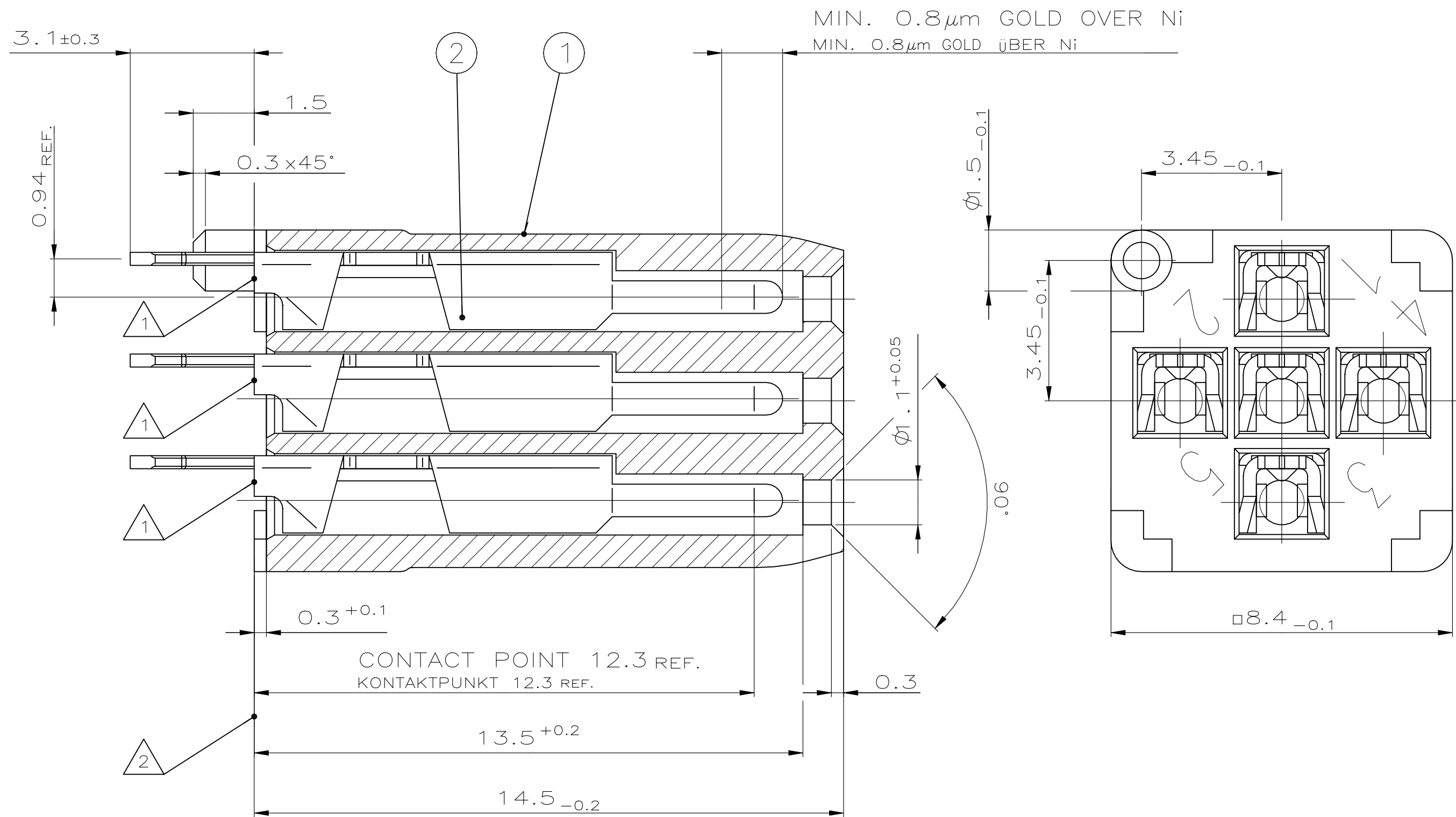
SECTION B-B
