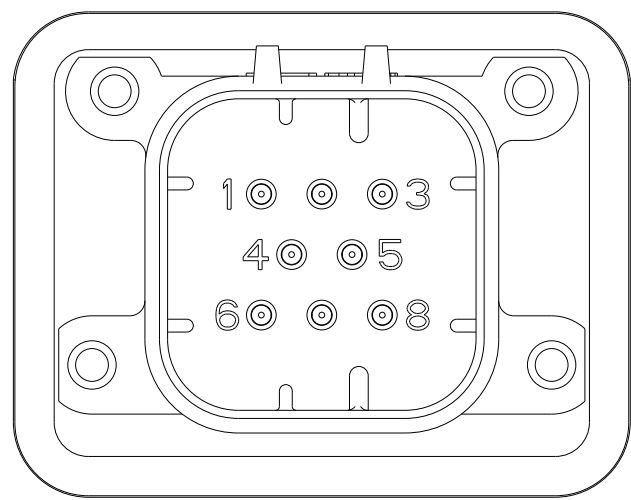
776280-1 & 1-776280-1 KEY LOCATION SCALE 2:1
