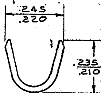
SECT. B-B
