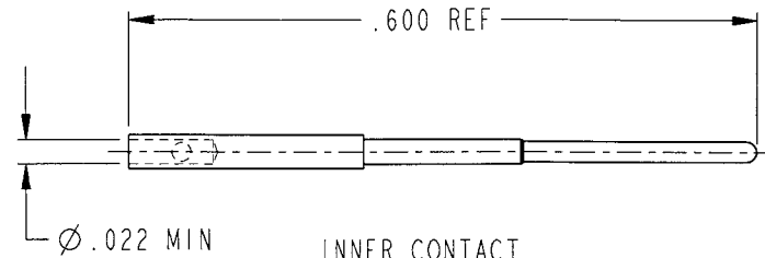
INNER CONTACT
