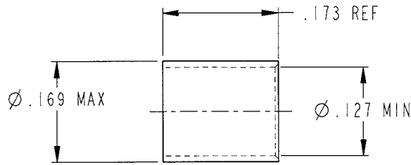
CRIMP FERRULE
