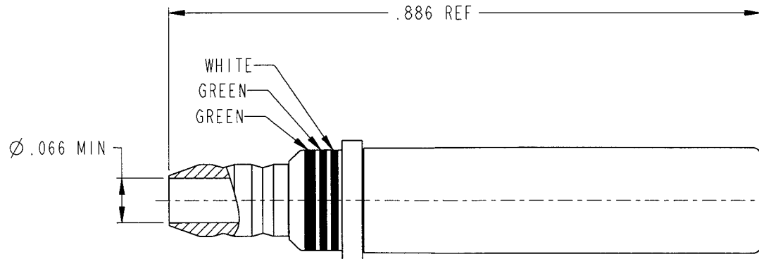
OUTER CONTACT
