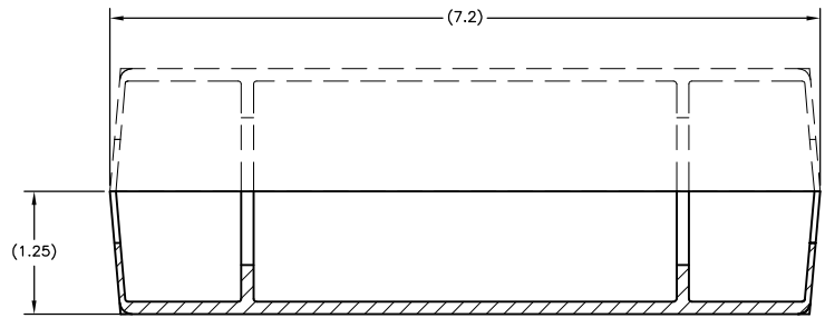
SECTION Z-Z
