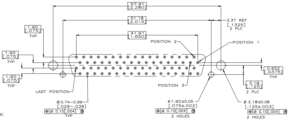
P.C. BOARD MOUNTING DIMENSIONS (CONNECTOR SIDE)
