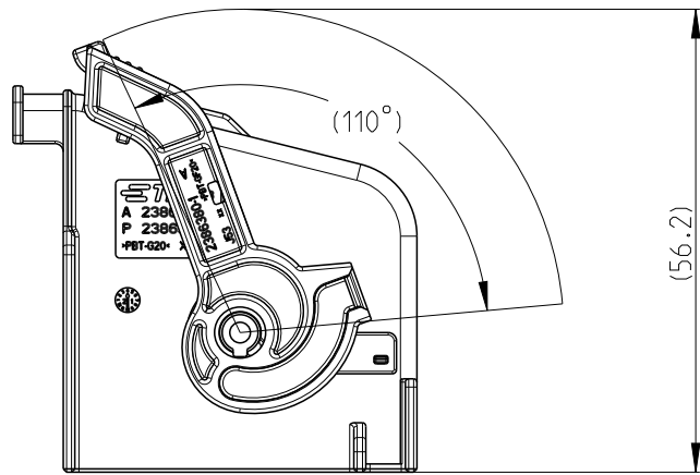
SCALE 1:1 LEVER IN LOCKED POSITION
