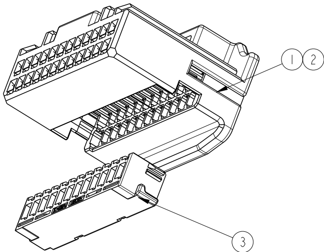
EXPLODED VIEW
