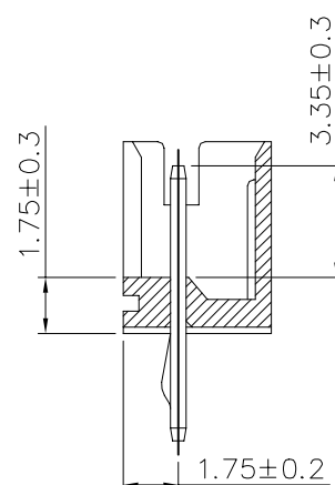
SECTION M-M
