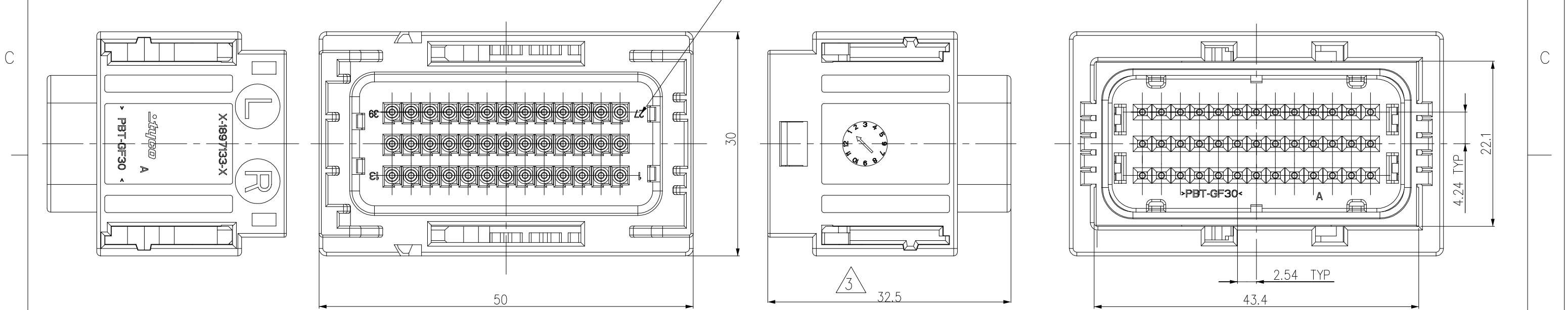
NOTE 1. GENERAL TOLERANCE : ±0.5 , ±3° 2. APPLICABLE CONTACT : SEE TABLE 1 3. SUPPLY CONDITION 4. SPACE OF ACTIVITY 5. USEABLE MATING PART HEADER ASSY : 1897129, 2005256, 200530, 2109430, 2219316, 2298790 COVER ASSY : 1897138-1, 2005535-1
