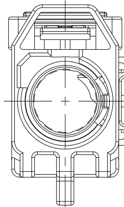
DETAIL E SCALE 3:1
