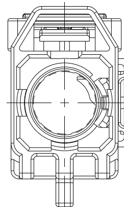
DETAIL Z SCALE 3:1
