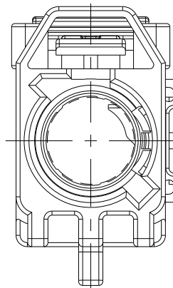
DETAIL G SCALE 3:1
