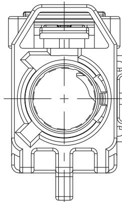
DETAIL F SCALE 3:1
