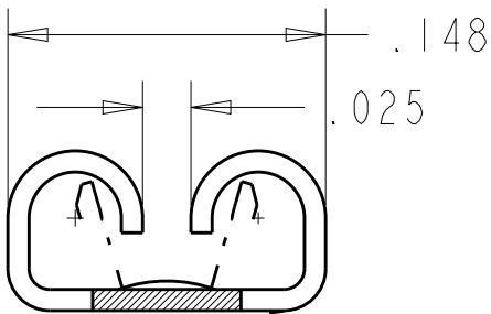
SECTION B-B SCALE 10:1
