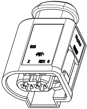
PERSPECTIVE VIEW SCALE 2:1
