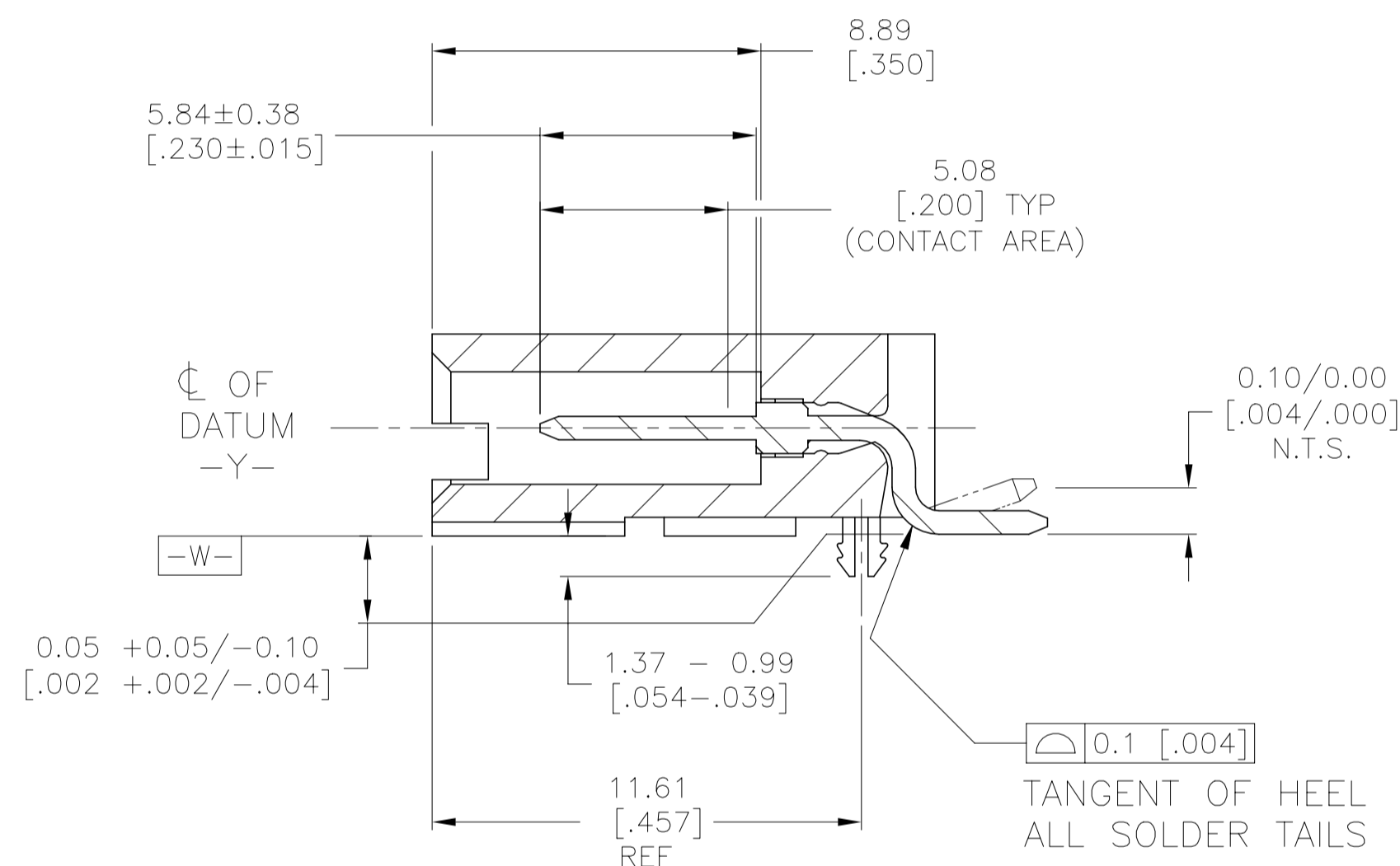
SECTION K-K
