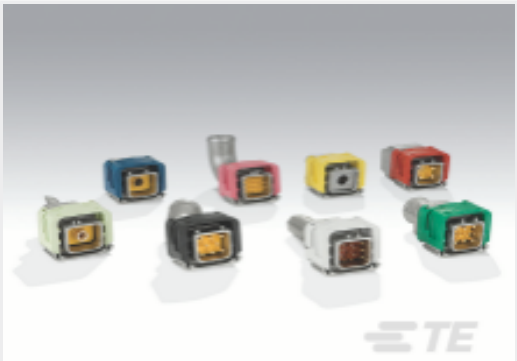
TE 产品编号CAT-DMC-MD-20 Rectangular Connector Plugs, Tool-less Assembly
