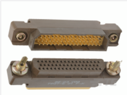
TE 产品编号ZPF000000000017887 FAST-E 03 M-X
