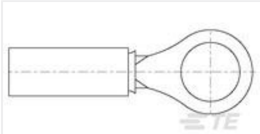
TE 产品编号1577624-1 TERMINAL RT PIDG PEEK STRATO 20 AWG
