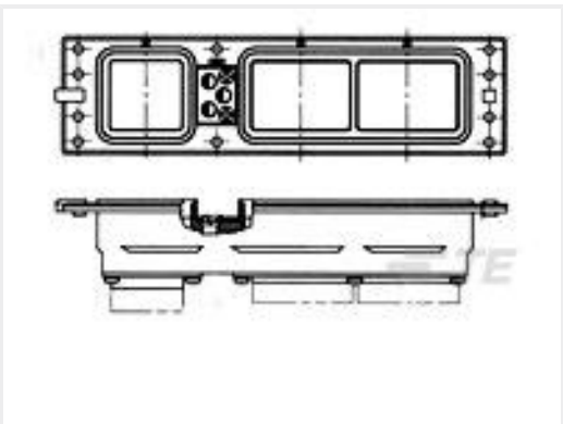
TE 产品编号448706-4 ASSY,CONN,RCPT,S22,ARINC 600
