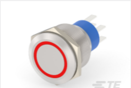
TE 产品编号6-2213772-5 AV22 DPL 3A MOVE RING LED RED 12V
