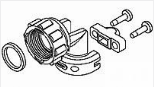
TE 产品编号YDTS26W17-35SNV001 PLUG ASSY
