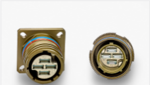
TE 产品编号1-2358899-3 conn .assy ,plug ,FO, MTsize15, 4cav
