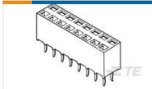
TE 产品编号215309-4 2X4P HV100 REC CON. TE, 8.5MM
