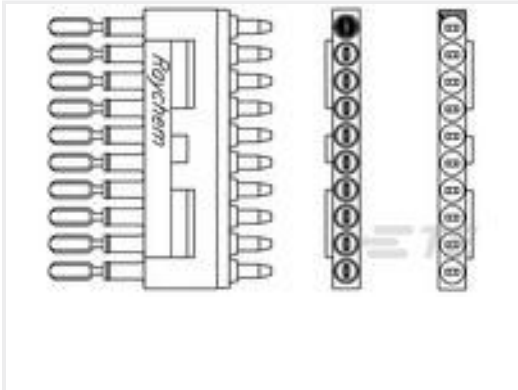
TE 产品编号699220-000 MTCB2X-XXX-206
